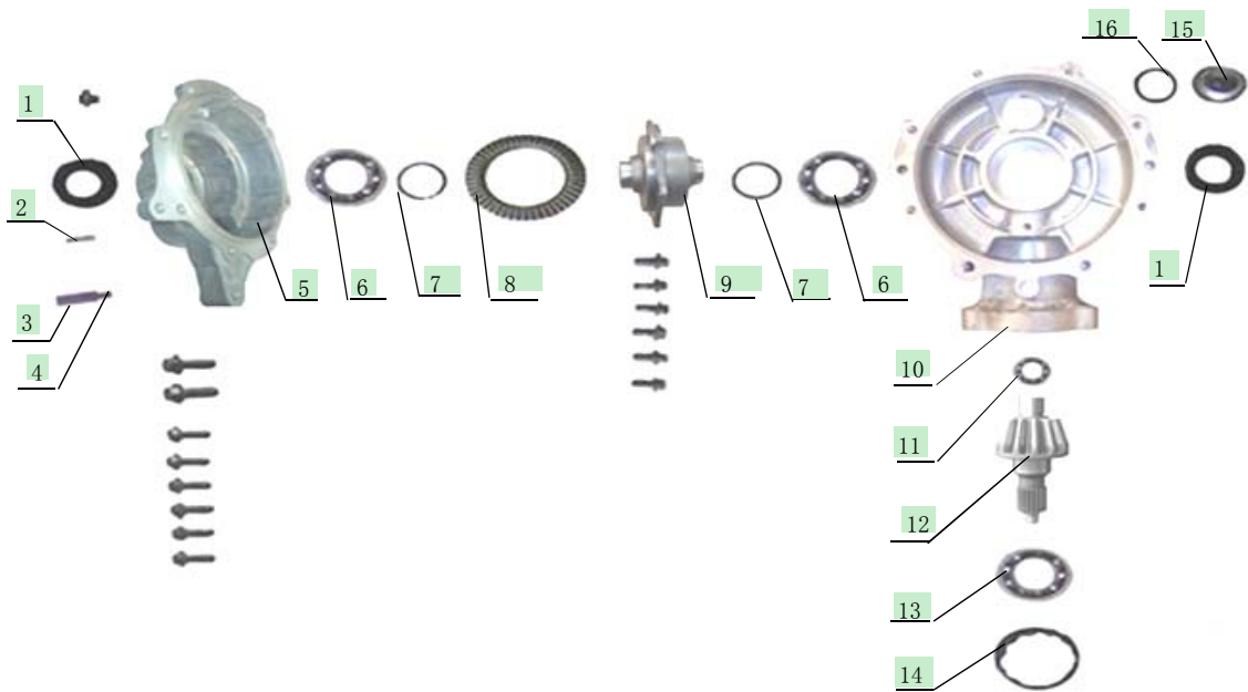
16、前减速器总成 Front Drive Reducer
