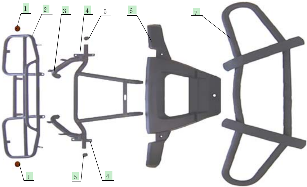
7、前货架总成 Front luggage carrier
