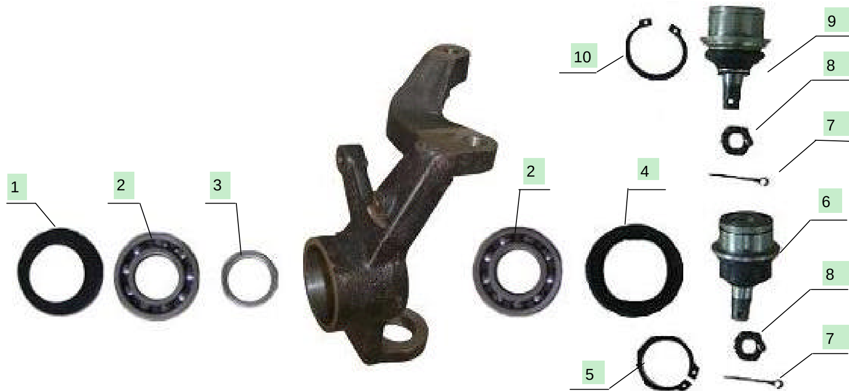
U4? Knuckle
