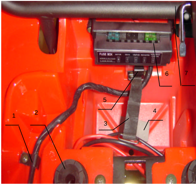
VI 30,BATERY INSTALLATIOIN
