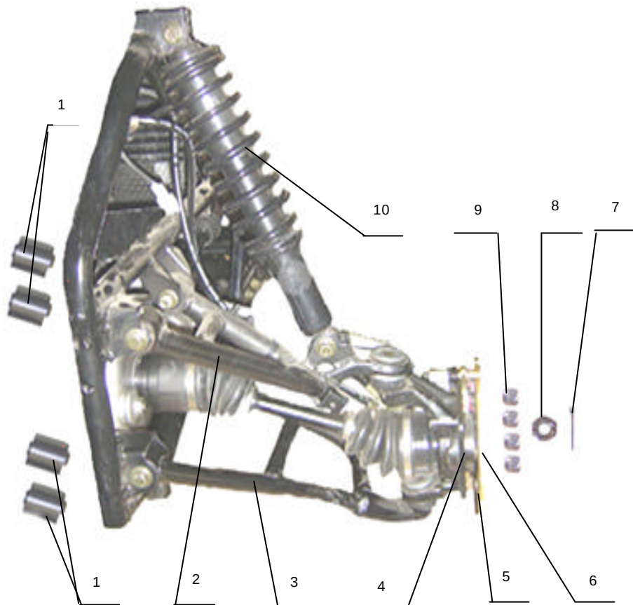
V I 2? Front suspension ASSY
