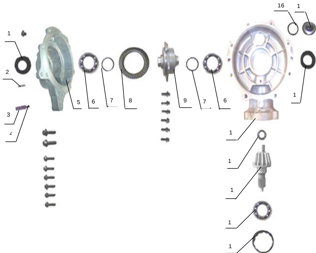
VI 16,FRONT DIFFERENTIAL ASSY
