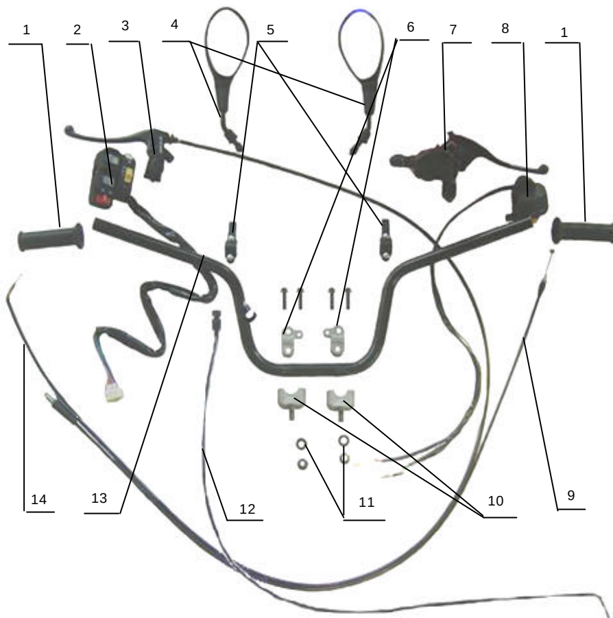
V 15 ,HAND BAR ASSY
