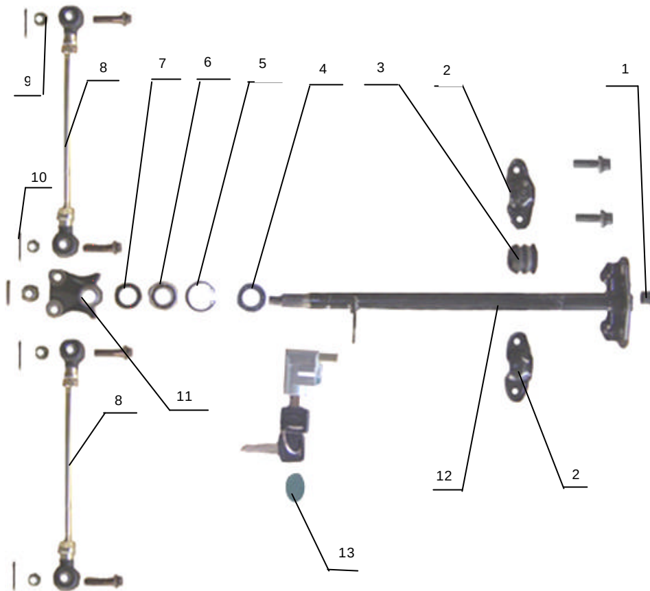
V I 4? STEERING SYSTEM
