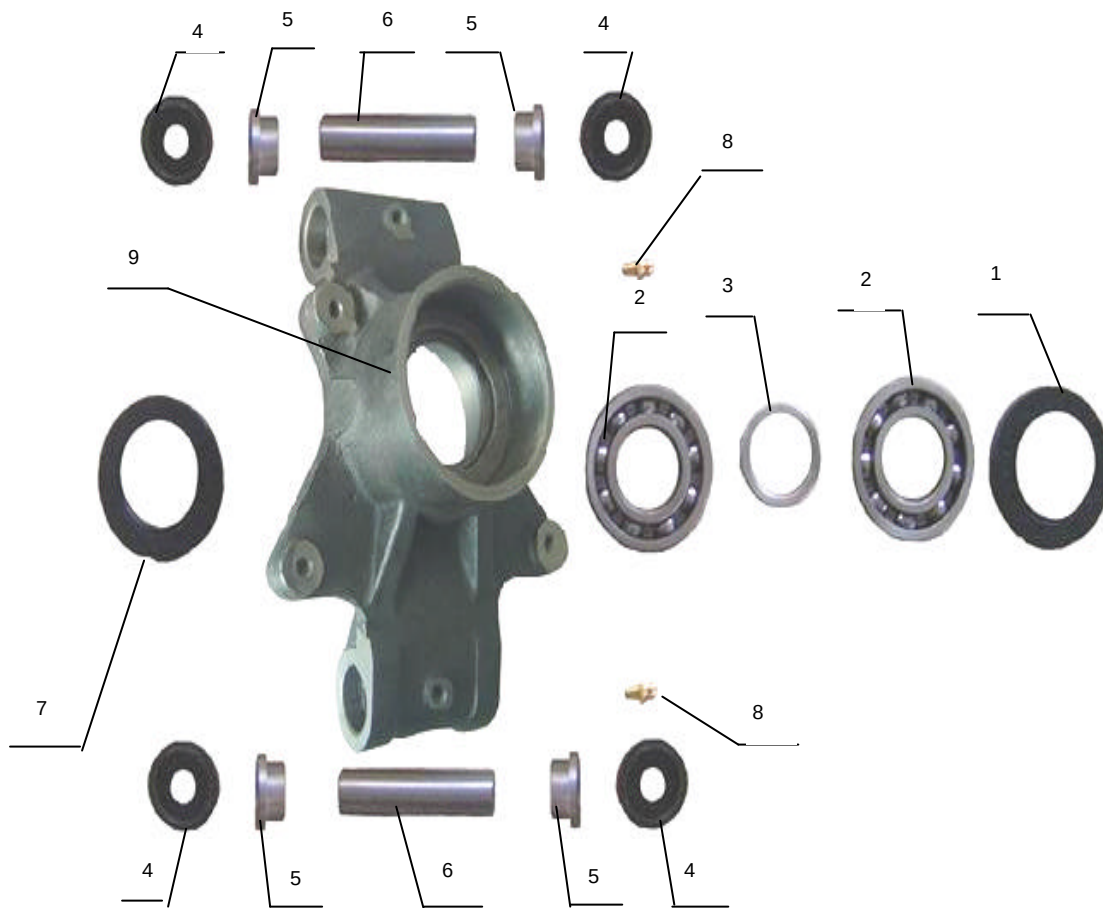
VI 19,SUPPORT ASSY
