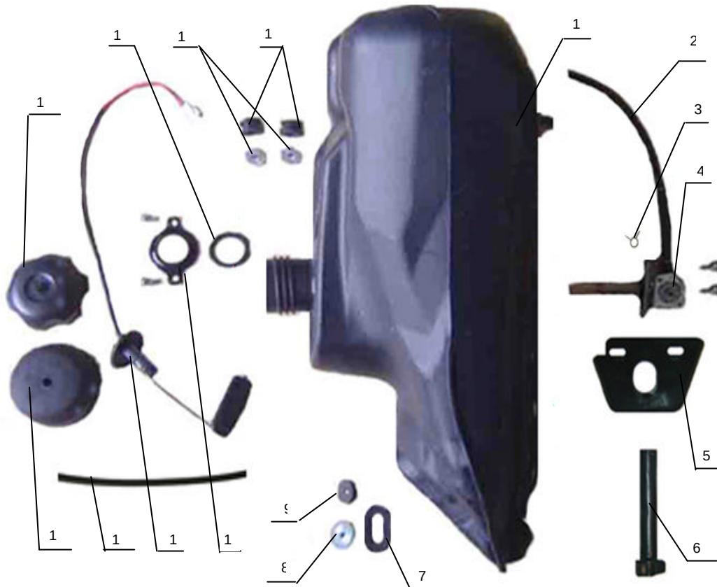
VI 31,FUEL TANK
