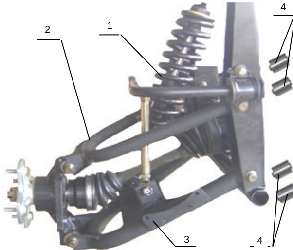
VI3? Front suspension ASSY
