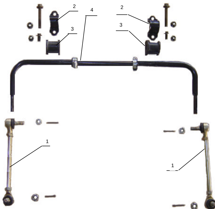
VI 9 TRANSVERSE STABILIZATION SUSPENSION
