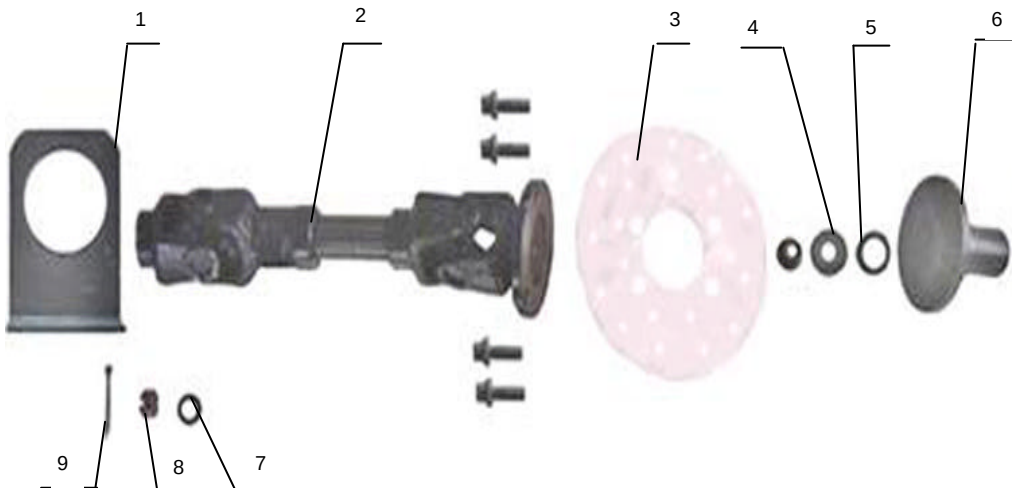
VI 13.,REAR TRANSMISSION ASSY
