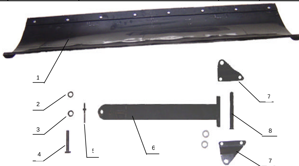
VV 37? SNOW PLOW ASSY
