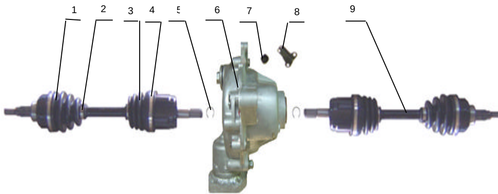
VI 14,FRONT DRIVE ASSY
