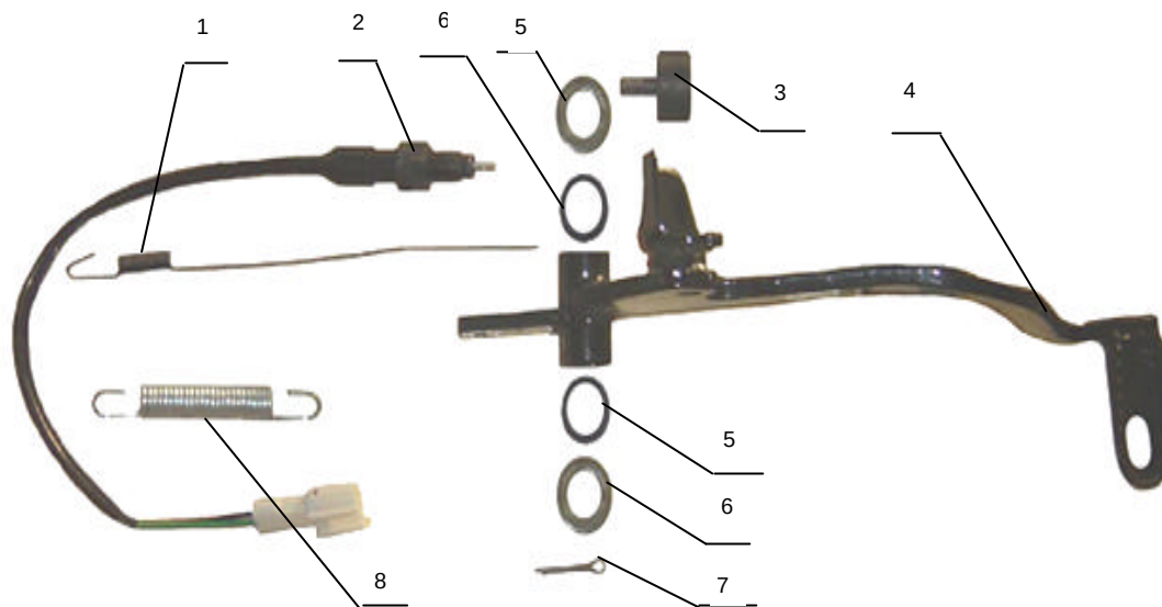
VI 34,BRAKE PEDAL ASSY
