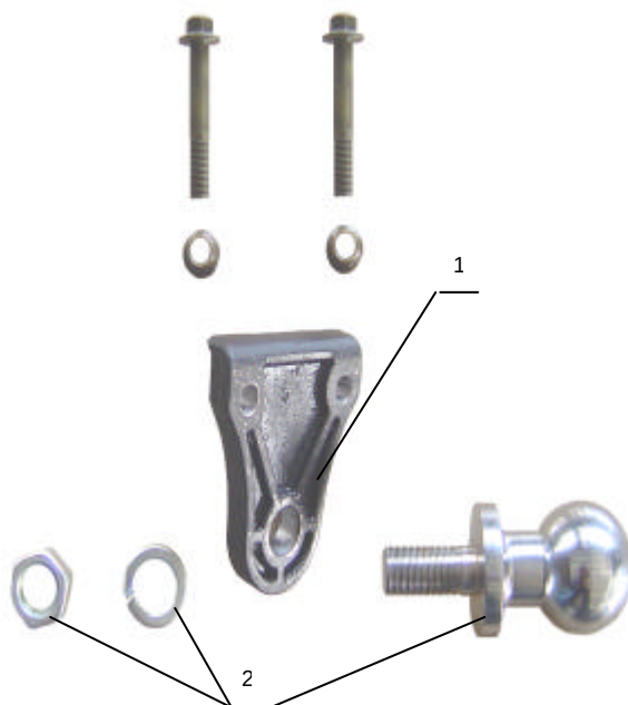
VI 10 TRAILER POTHOOK ASSY
