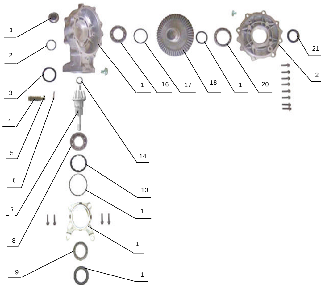
VI 17,REAR DIFFERENTIAL ASSY
