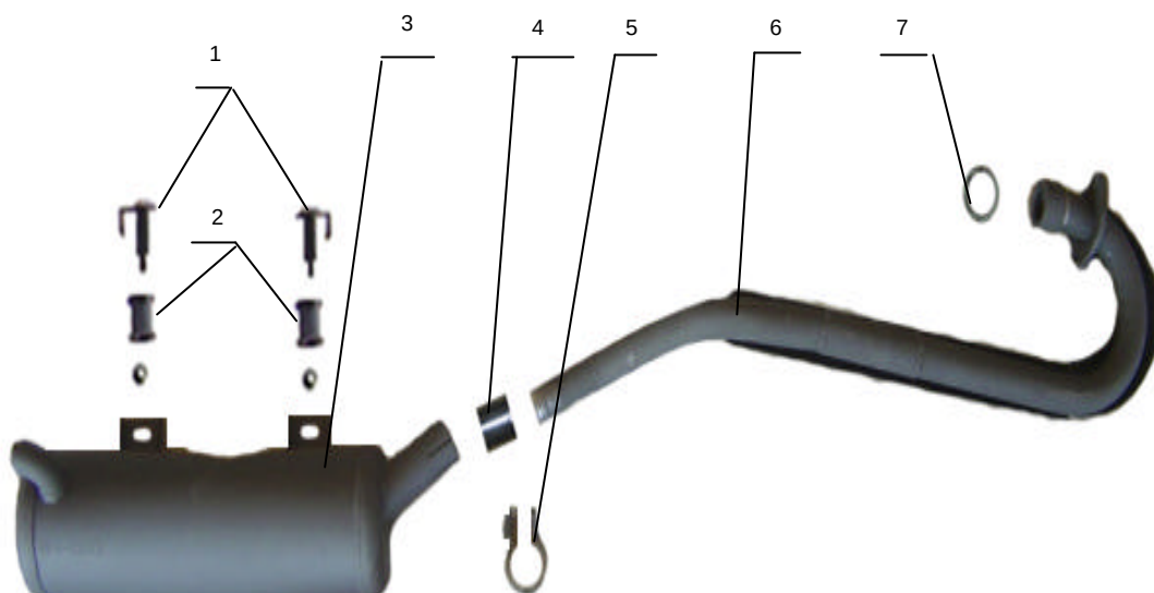
VI 32,EXHAUST SYSTEM
