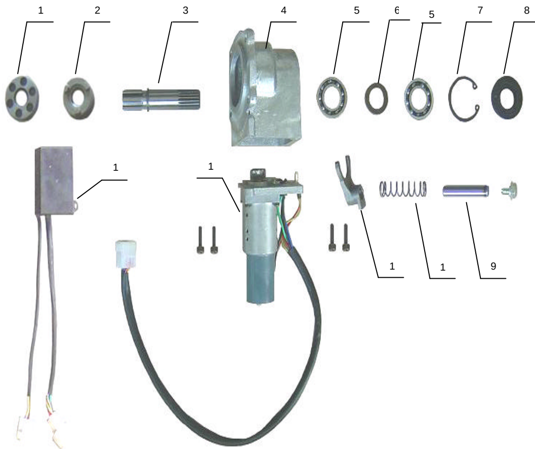
VI 11 2WD/4WD SELECTABLE ASSY
